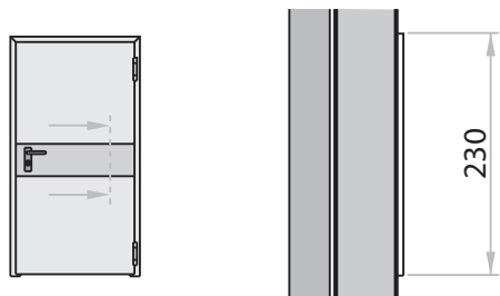
Protection plates
